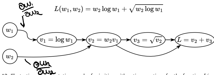
Рис. 12: Illustration of computation graph of primitive arithmetic operations for the function L(w_1, w_2)
