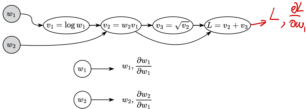
Рис. 7: Illustration of forward mode automatic differentiation
