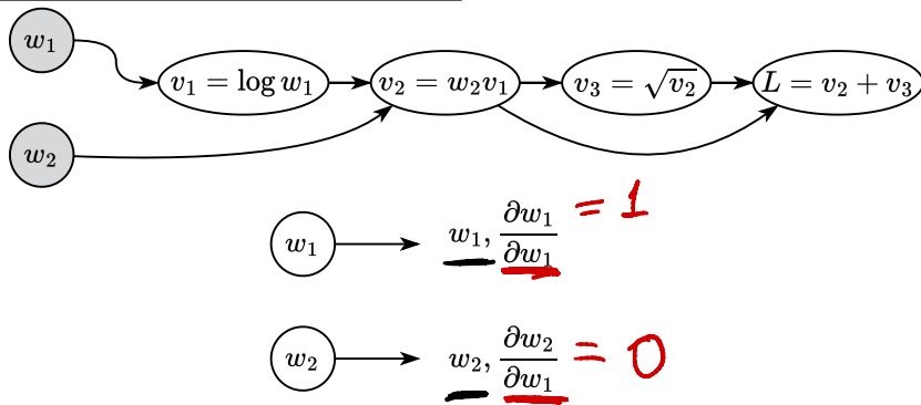
Рис. 7: Illustration of forward mode automatic differentiation
