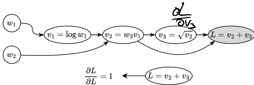
Рис. 20: Illustration of backward mode automatic differentiation
