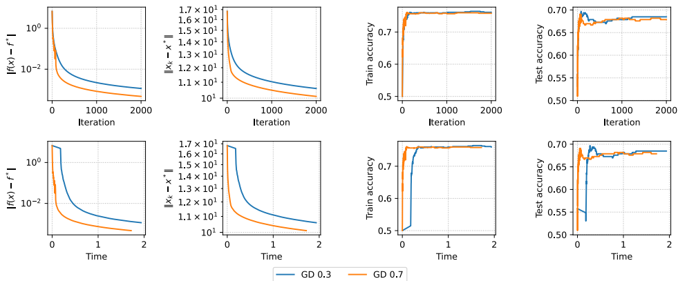
Figure 23: Only small precision is achievable with sublinear convergence
