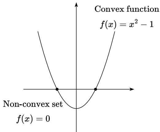
Figure 25: The idea behind the definition of a convex optimization problem
