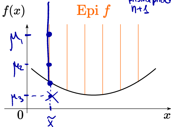
Figure 10: Epigraph of a function
