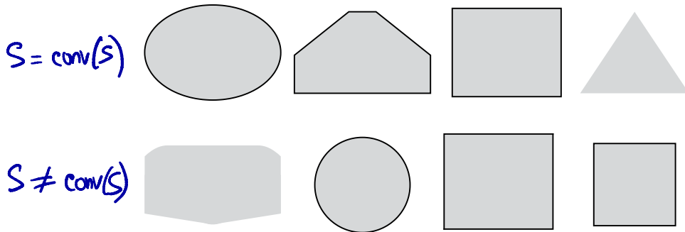
Figure 6: Top: convex hulls of the convex sets. Bottom: convex hull of the non-convex sets.
